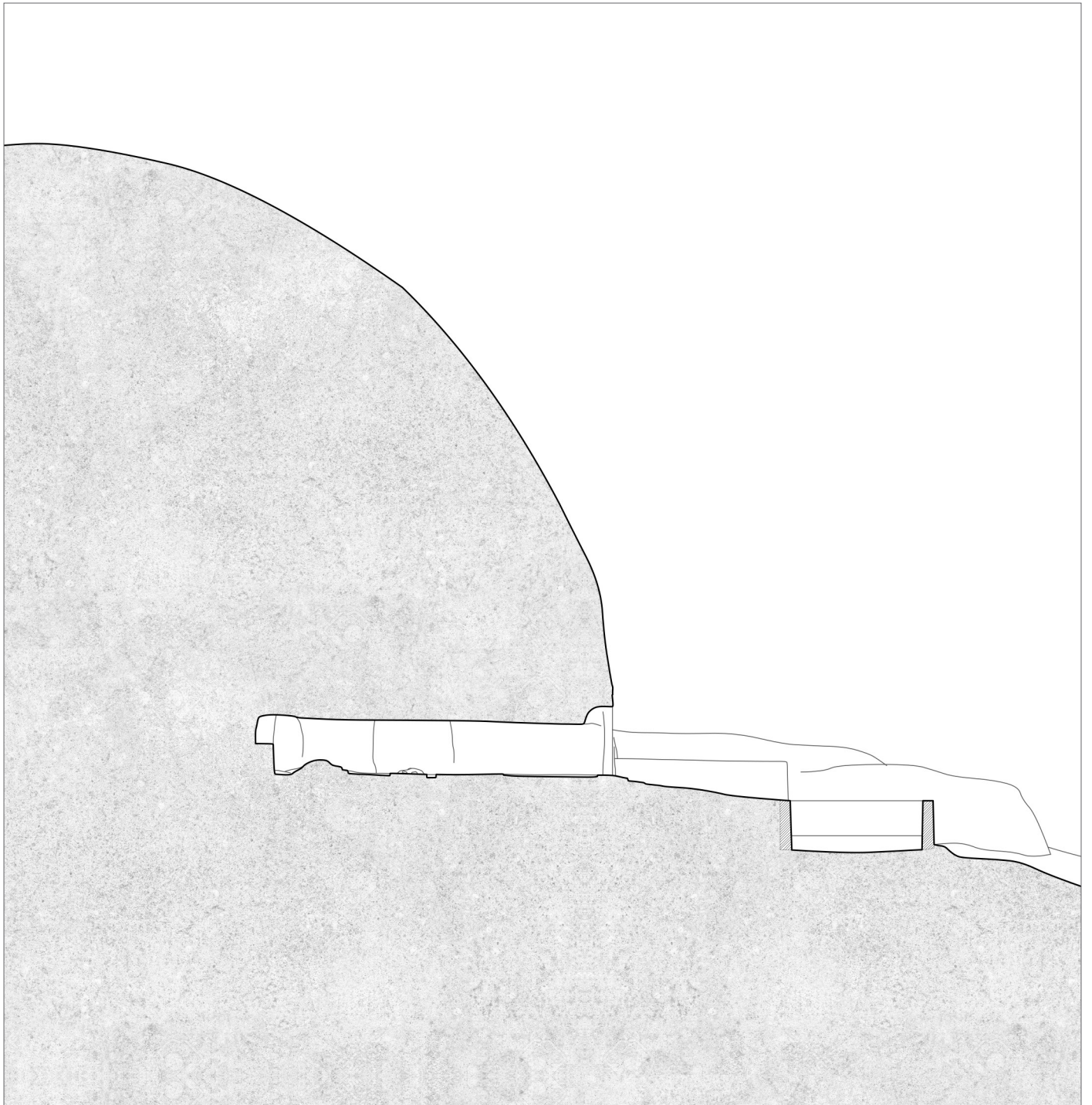
Arbatu Ensesa Be'era Section BB (2016)
